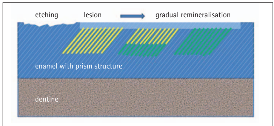
Fig. 1 Schematic of cross section of tooth depicting structural changes occurring during tooth erosion, and de- and remineralisation (from left to right). With erosion an integral layer of enamel is removed by strong acids; this layer is not restored after the pH is returned to neutrality. In contrast, weak organic acids formed in dental plaque, when sugars are metabolized, lead to preferential dissolution in the spaces between the enamel prisms. These acids bypass the fluoride rich outer enamel layer. When pH return to neutrality calcium and phosphate ions from saliva can precipitate in these dissolved regions. In the presence of fluoride this leads to an enforced mineral, less susceptible to future acid attacks.
