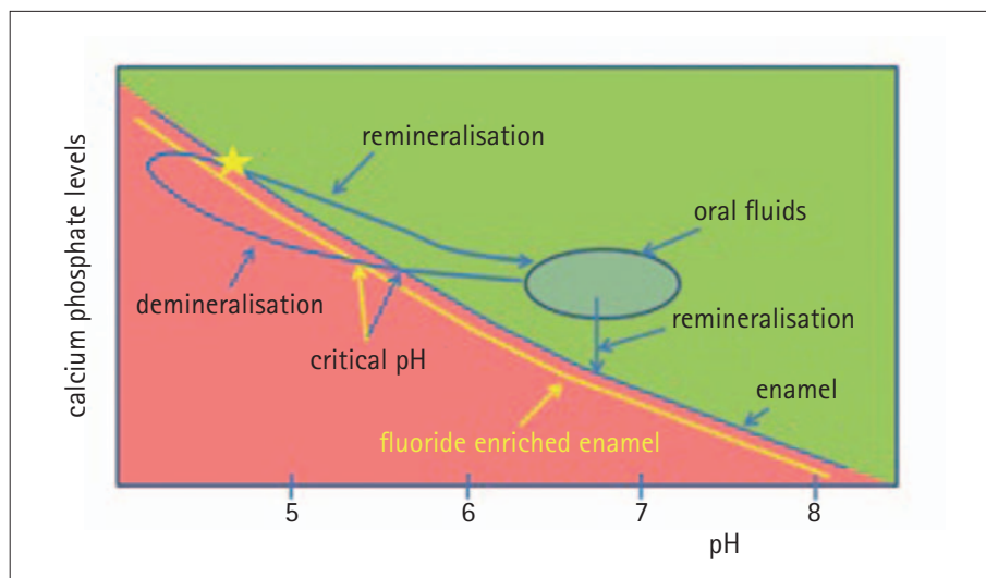
Fig. 3 Graph depicting the primary modes of action of fluoride: decreasing demineralisation and enhancing of remineralisation. Solubility of hydroxyapatite (HAP) depends on pH of the oral fluids (plaque). At physiological pH (6–7), the calcium and phosphate levels are supersaturated with respect to HAP and can lead to remineralisation (green region). When acids are formed in the plaque, the pH decreases and beyond the critical pH this leads to dissolution of HAP (red region). This leads to an increase of the calcium and phosphate levels. When all sugars are metabolised and pH is increased due to salivary buffering (and HAP dissolution) the return part of the cycle is started. At some stage (see star) mineral will start to reprecipitate. The presence of fluoride leads to lower solubility (see yellow line), hence a lower (critical) pH at which dissolution starts, and a lower pH at which mineral reprecipitation occurs
