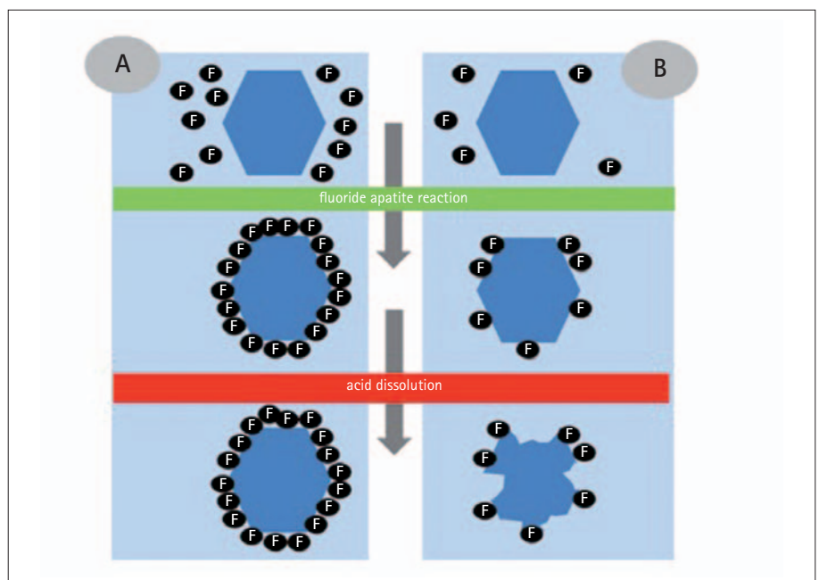
Fig. 2 Events taking place at the surface of hydroxyapatite crystallites. Fluoride-ions are adsorbed onto the crystals. Full coverage (A) will prevent dissolution of the crystallites during an acid attack. Partial coverage (B) will lead to partial dissolution (modified from Arends and Christoffersen, 32 and Buzalaf et al. 33 )
