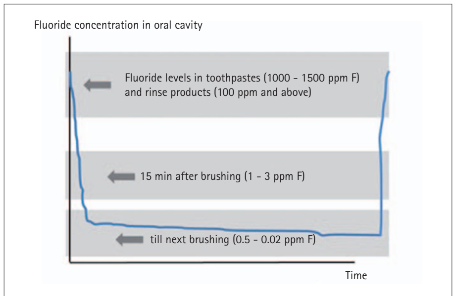
Fig. 4 Schematic of fluoride levels in the oral cavity after brushing or rinsing with a fluoride product. The fluoride concentration decreases sharply within minutes of using a product. The residual elevation still helps to promote remineralisation of the dental hard tissues
